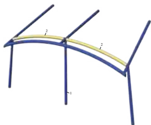
Octavia Air main frame system (additional roof support and storm tubes are supplied as standard on sizes 10-19)
